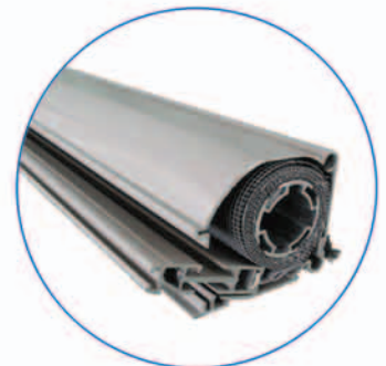
Window Screens - Complete Housing
